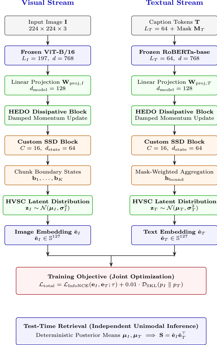
Fig. 1 Overall architectural pipeline of the proposed HEDO-HVSC multimodal state-space framework. Visual patch sequences ( L_I = 197 ) and textual token sequences ( L_T = 64 ) are extracted from frozen ViT-B/16 and RoBERTa-base encoders, projected to d_{\text{model}} = 128 , stabilized via HEDO coordinate-momentum dissipation, and processed through custom chunk-wise SSD recurrence blocks ( C = 16, d_{\text{state}} = 64 ). During training, mask-weighted boundary states parameterize Gaussian latent distributions regularized via symmetric KL divergence \mathcal{D}_{\text{SKL}} alongside multi-positive InfoNCE contrastive alignment. At test time, retrieval evaluates deterministic posterior means strictly unimodally with zero cross-modal communication.
