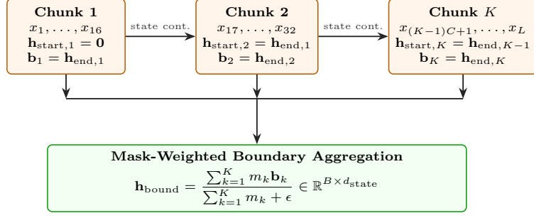
Fig. 3 State-continuous chunk-wise SSD-style recurrence with boundary state extraction. Recurrent hidden states propagate continuously across chunk boundaries ( \mathbf{h}_{\text{start},k} = \mathbf{h}_{\text{end},k-1} ) with zero state resets, while mask-weighted aggregation prevents zero-padding bias.
