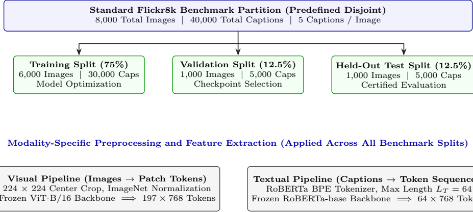
Fig. 5 Predefined Flickr8k dataset partition and modality-specific feature extraction pipeline. The 8,000 photographic images and 40,000 human-annotated captions are partitioned into verified disjoint training (6,000), validation (1,000), and held-out test (1,000) splits with zero cross-split leakage, followed by independent visual (ViT-B/16) and textual (RoBERTa-base) feature extraction.
