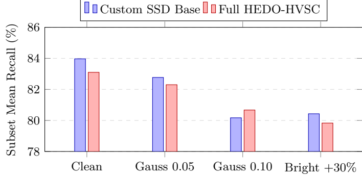
Fig. 7 Robustness comparison under pixel-space perturbations on a 100-image test subset. The evaluation exhibits a mixed robustness profile: Full HEDO-HVSC improves over the baseline under severe Gaussian noise ( \sigma = 0.10 , +0.50\% ), but achieves lower recall under the other tested conditions.
