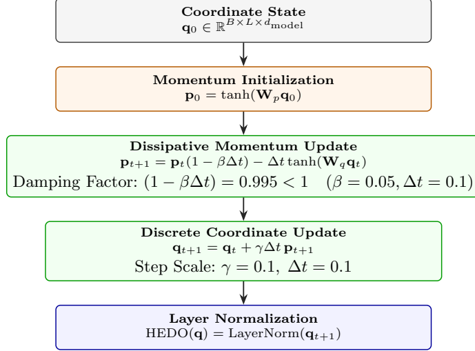
Fig. 2 Computational flow of the Hamiltonian-Inspired Energy Dissipation Operator (HEDO). Coordinate representations \mathbf{q}_0 initialize conjugate momenta \mathbf{p}_0 . Discrete updates execute damped momentum updates (1 - \beta\Delta t) = 0.995 and discrete coordinate updates before Layer Normalization.
