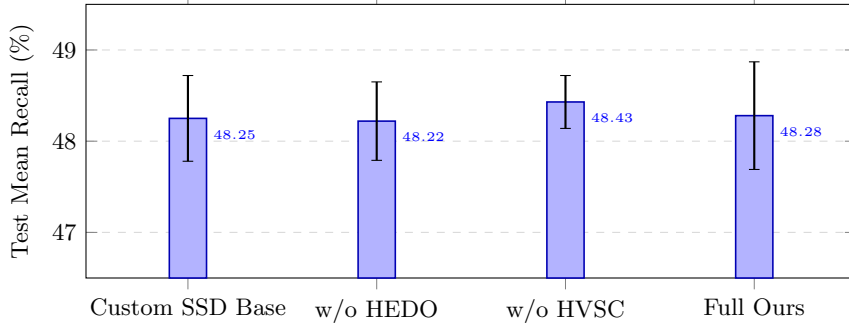
Fig. 6 Controlled 4-model factorial benchmark comparison across 3 independent random seeds (42, 43, 44) on the standard Flickr8k predefined held-out test split ( N = 1,000 images, 5,000 captions). Error bars represent \pm 1 standard deviation.
