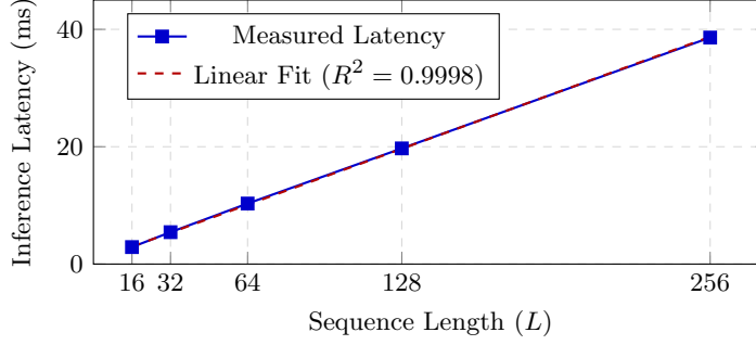
Fig. 8 Empirical inference latency scaling of the custom PyTorch chunk-wise SSD block ( d_{\text{model}} = 128, d_{\text{state}} = 64, B = 16 ). Measurements exhibit approximately linear empirical latency scaling over the tested sequence lengths.
